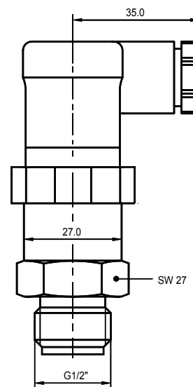
P 10 / P 21 G1/2" 1.4404
